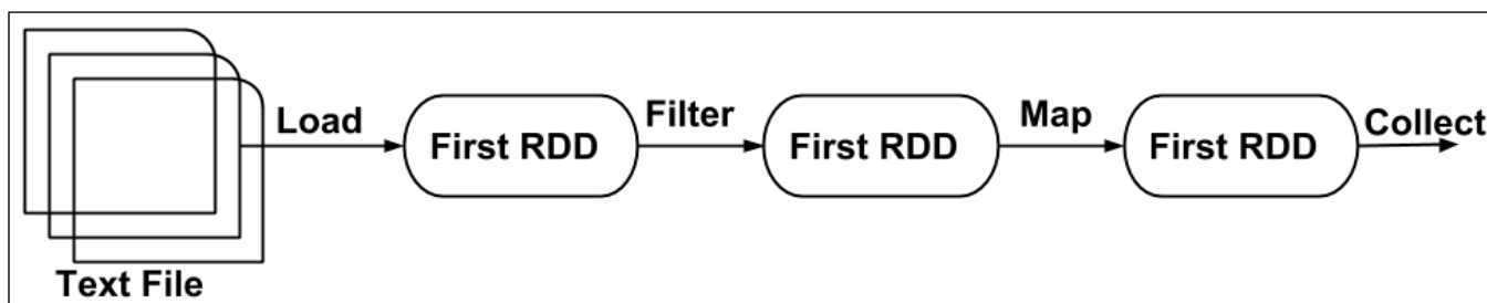
Figure 1. RDD transformations.
