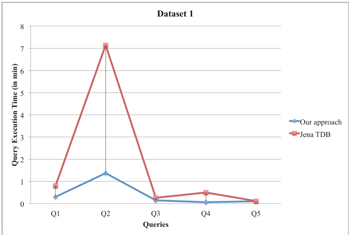
Figure 11. Query comparison.
