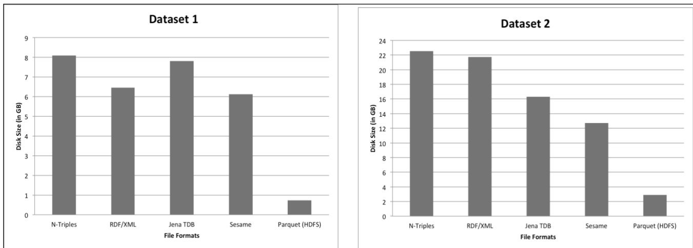
Figure 9. Disk size for different file formats.
