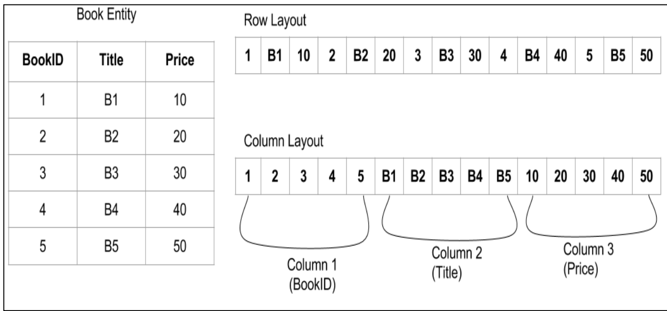
Figure 3 An example of an entity and its row and column representation.
