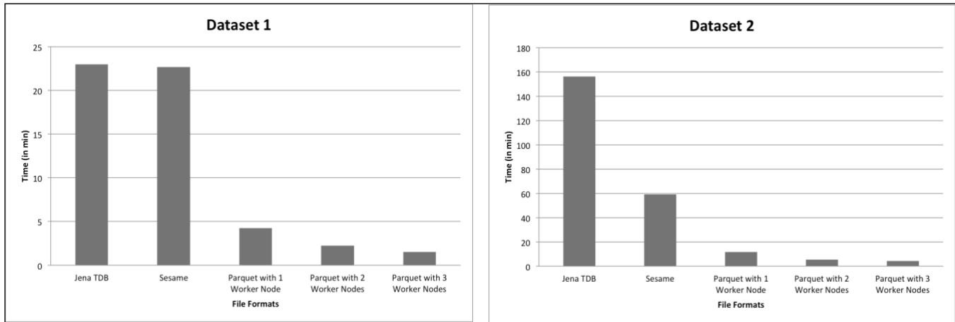
Figure 8. Data storage time for different file formats.
