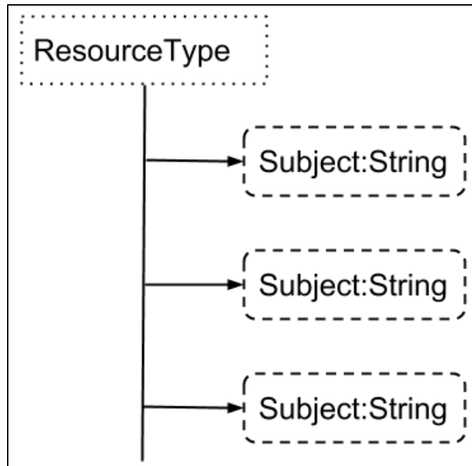
Figure 5. RDF Triple view.
