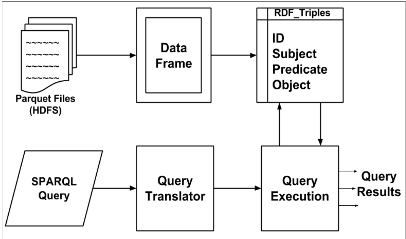
Figure 7. Process of query execution.
