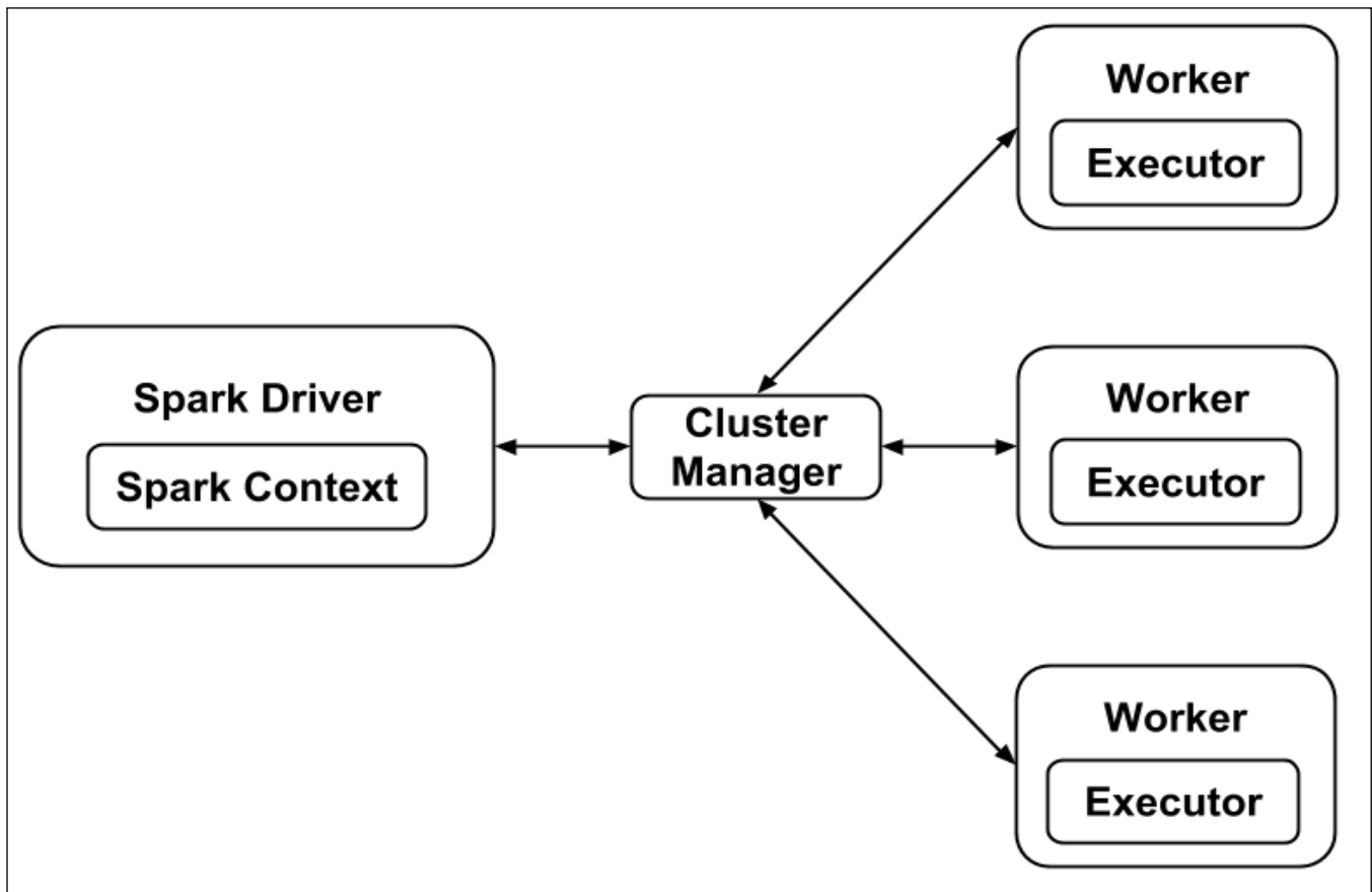
Figure 2 Execution model of Spark.
