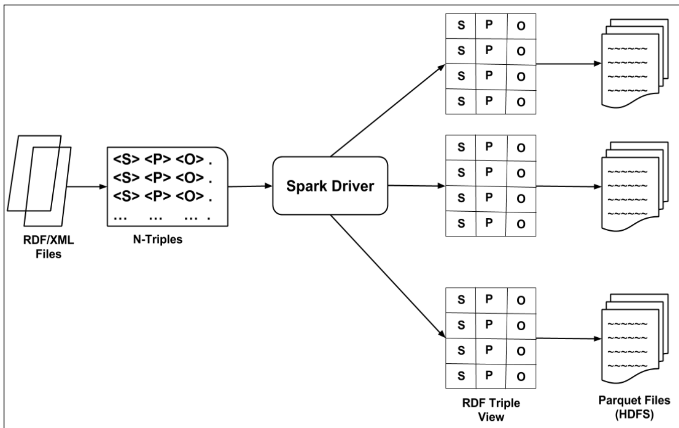
Figure 6. Data-storing process in HDFS.
