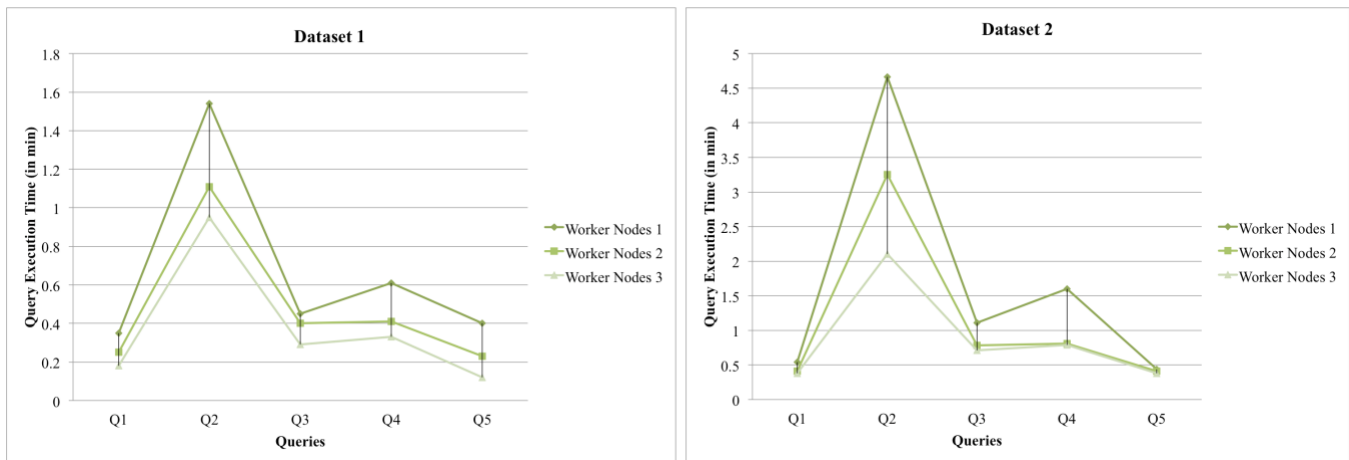
Figure 10. Query response time with different numbers of worker nodes.
