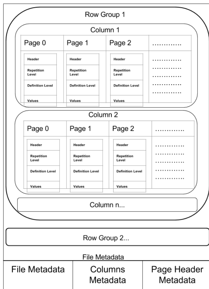
Figure 4 Parquet file structure.
